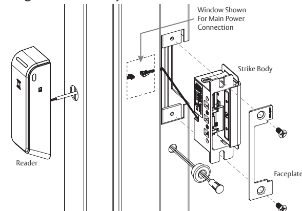
Diagram 6 Wiring
