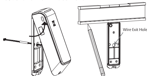
Diagram 2 Remove Back Cover and Mark Placement
