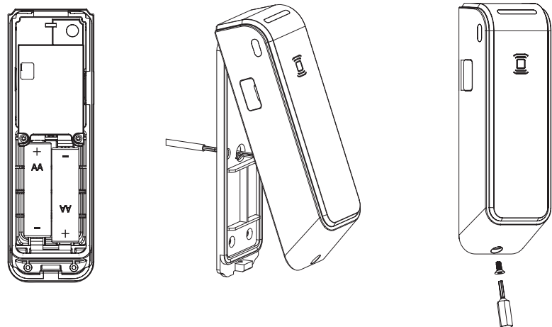
Diagram 9 Install Batteries & Secure Reader
