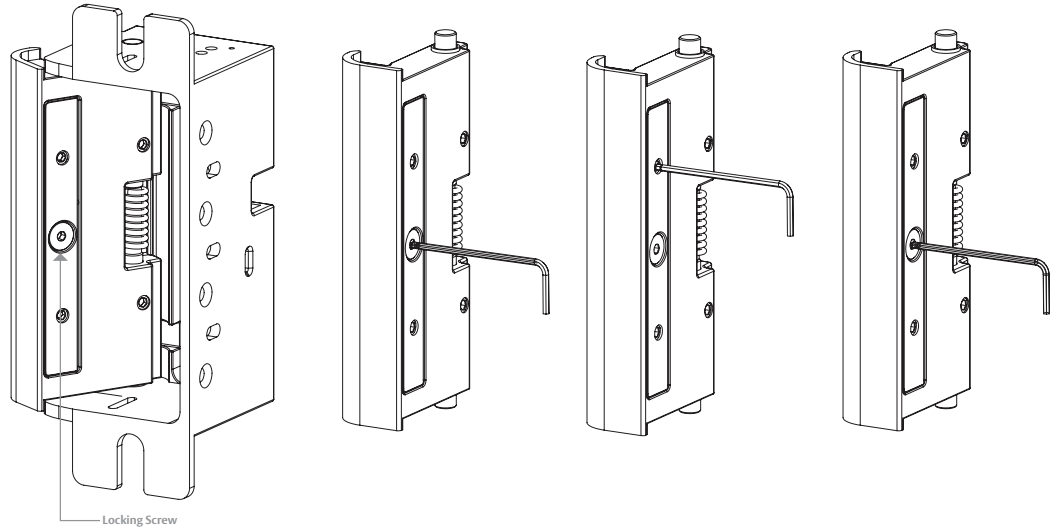
Diagram 7 Adjusting the Horizontal
