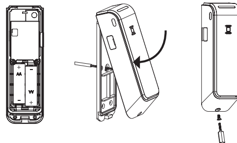
Diagram 5 Assembly
