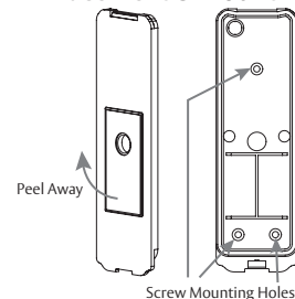
Diagram 3 Placement & Mounting
