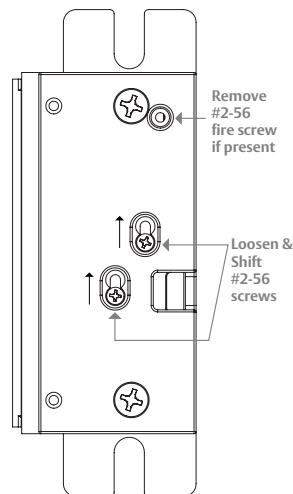
Diagram 3: #2-56 screws
