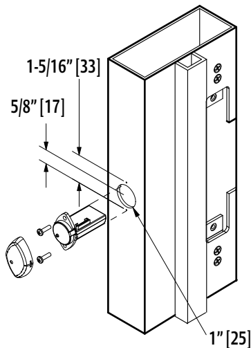
Reader/Antenna
